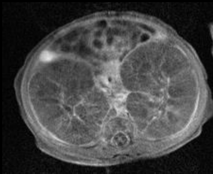
T1-weighted image post gad
